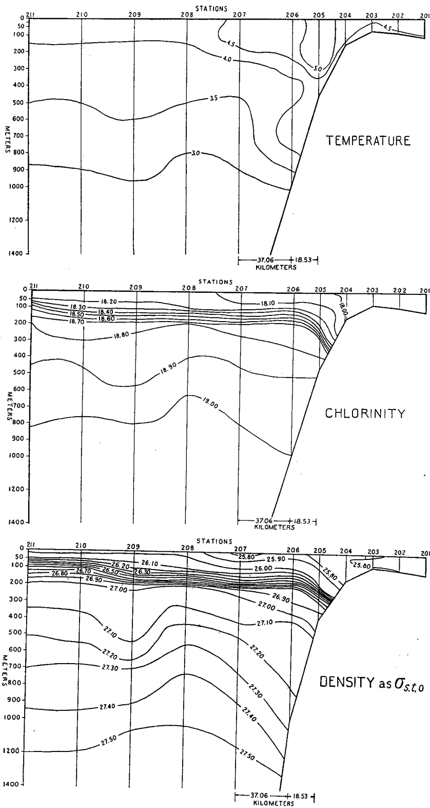
FIGURE 5.—Diagram of distribution of Temperature, Chlorinity, and Density as \sigma_{s, t, \rho} for Cape Chiniak Section.
