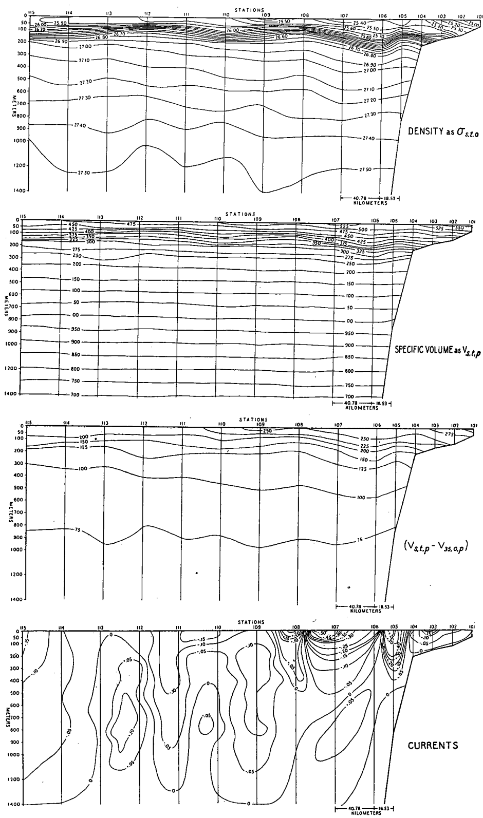
FIGURE 4.—Diagram of distribution of the specific volume as V_{s,t,p} , its anomaly (V_{s,t,p} - V_{s,\theta,p}) , and the currents in knots in the Cape Clear Section.
