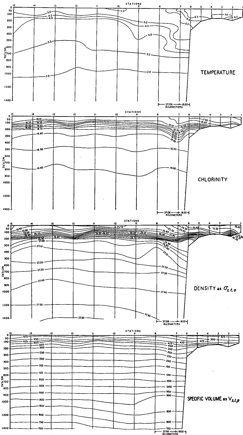
FIGURE 1.—Diagram of distribution of Temperature, Chlorinity, and Density as \sigma_{s,t,o} for Ocean Cape Section.
