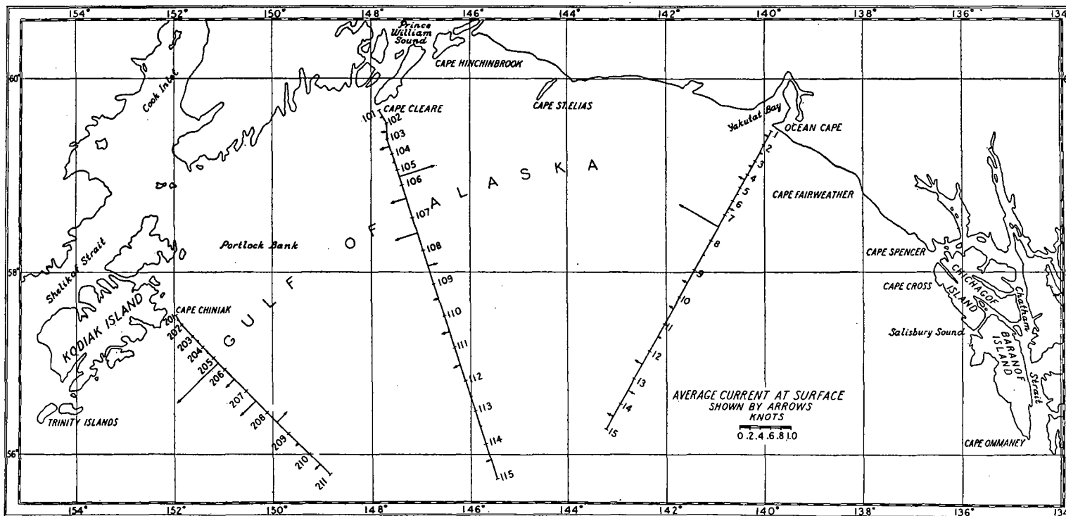
FIGURE 7.—The average current at the surface of Ocean Cape, Cape Cleare, and Cape Chiniak Sections in January.
