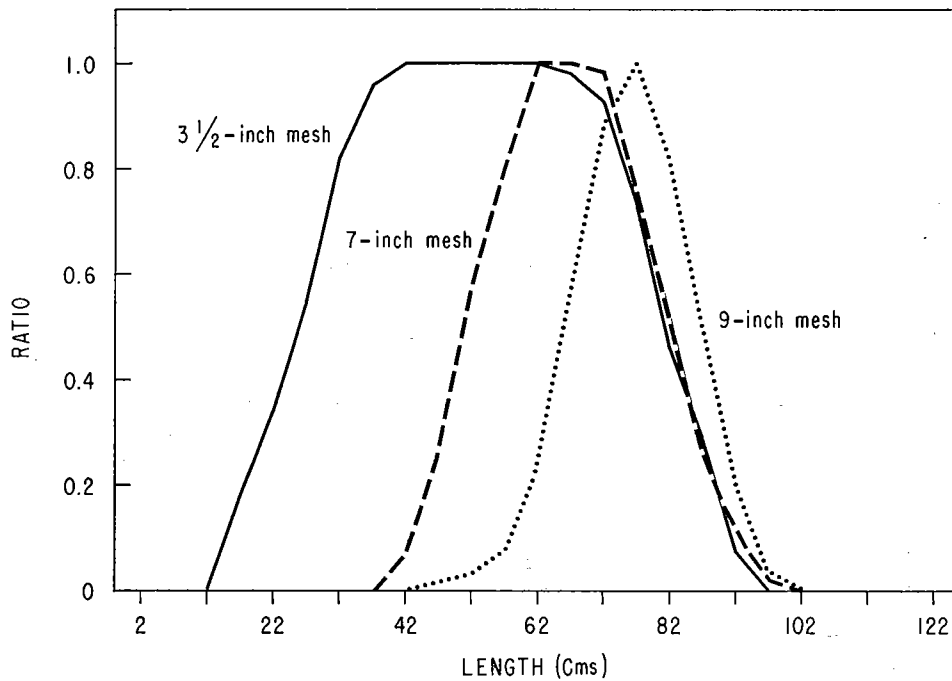
Figure 8. Calculated total selection curves for trawl nets having 3½-, 7- and 9-inch codend meshes.
