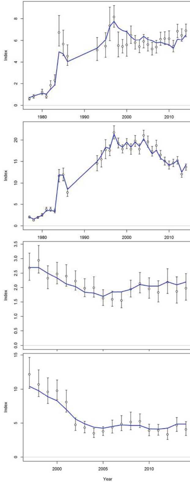
Figure 61. Fit to the index of abundance from the survey (numbers-per-unit-effort) for Area 2 (upper panel), Area 3(second panel), Area 4 (third panel) and Area 4B (bottom panel) in the AAF long model.
