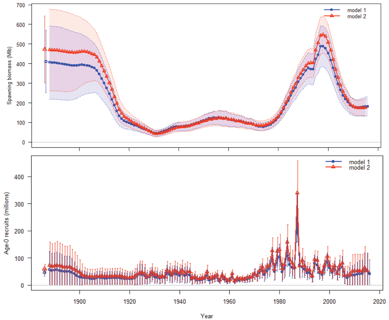
Figure 39. Comparison of spawning biomass (upper panel) and recruitment (lower panel) from the 2014 and preliminary 2015 coastwide long models including all updates to data and model structure.
