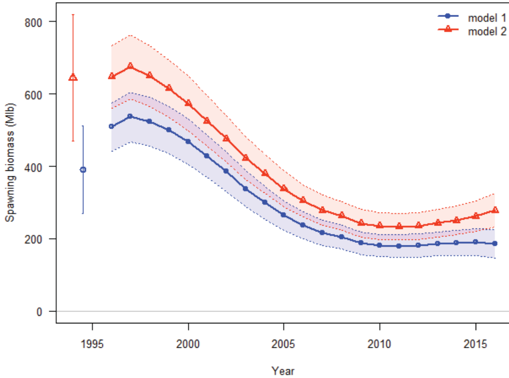
Figure 90. Comparison of the AAF short model (upper series) and the CW short model (lower series).
