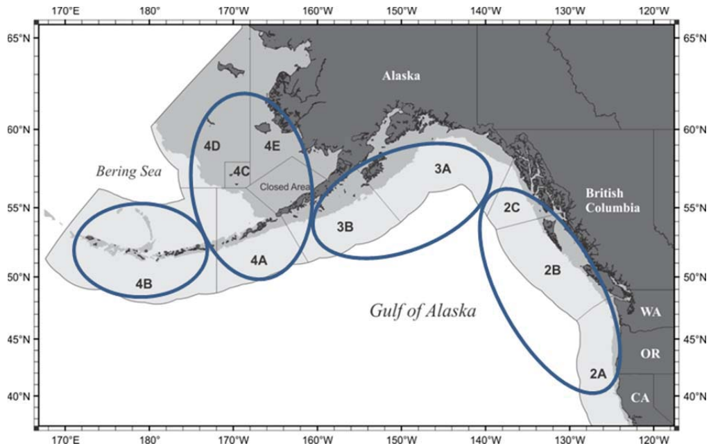
Figure 1. Current IPHC regulatory areas. Shaded region denotes the Exclusive Economic Zones of the U.S. and Canada. Circles denote aggregated geographic areas (2, 3, 4, and 4B) used to partition the data in the AAF models.
